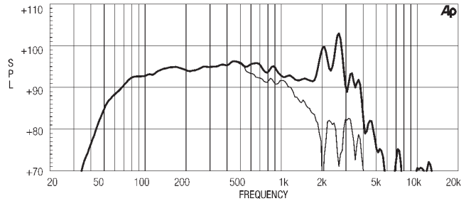
FREQUENCY RESPONSE CURVE OF 12LW801 MADE ON 50 LIT. ENCLOSURE TUNED 60HZ IN FREE FIELD (4PI) ENVIRONMENT. ENCLOSURE CLOSES THE REAR OF THE DRIVER. THE THIN LINE REPRESENTS 45 DEG. OFF AXIS FREQUENCY RESPONSE.
